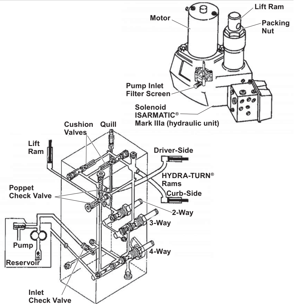
HYDRAULIC SYSTEM
