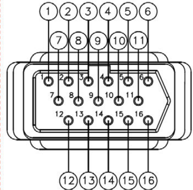
VEHICLE SIDE 72546
